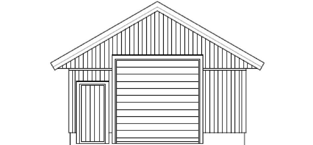
FASAD GAVEL
